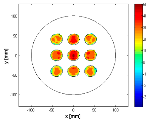
Figure 5. The magnitude of electric fields on each aperture.
