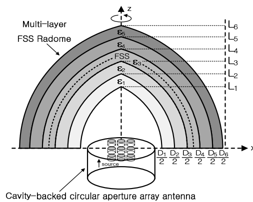
Figure 1. Problem geometry.
