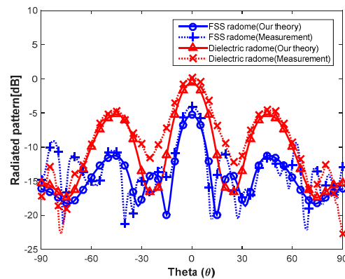
Figure 9. The dielectric and FSS radome enclosing the 3 \times 3 cavity-backed circular aperture array antenna ( \varphi = 0^\circ ).
