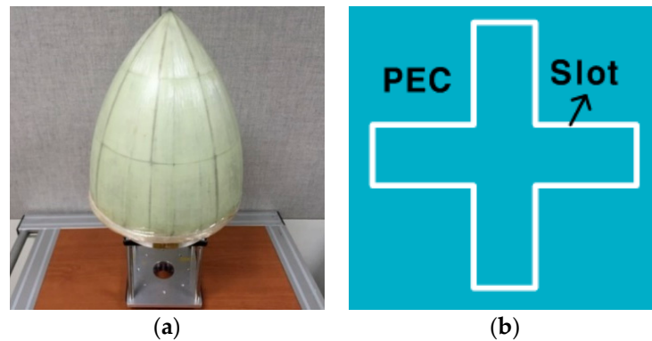
Figure 7. (a) The FSS radome and (b) the unit cell of the FSS layer.
