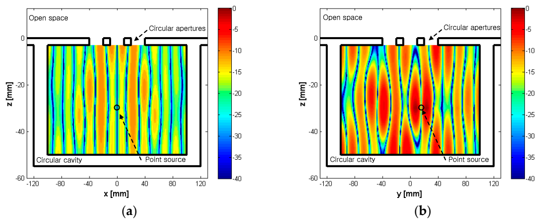
Figure 4. Normalized internal (within the cavity) magnetic field in dB scale at 10 GHz. (a) H_y ( xz -plane), (b) H_x ( yz -plane).
