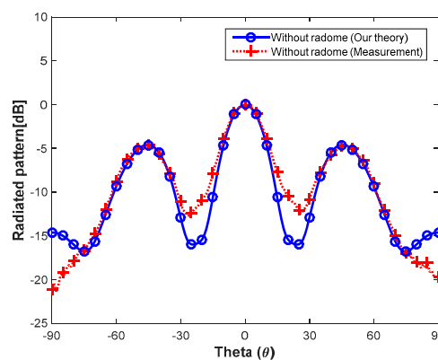
Figure 6. Radiation pattern of the 3 \times 3 cavity-backed circular aperture array antenna ( \varphi = 0^\circ ).
